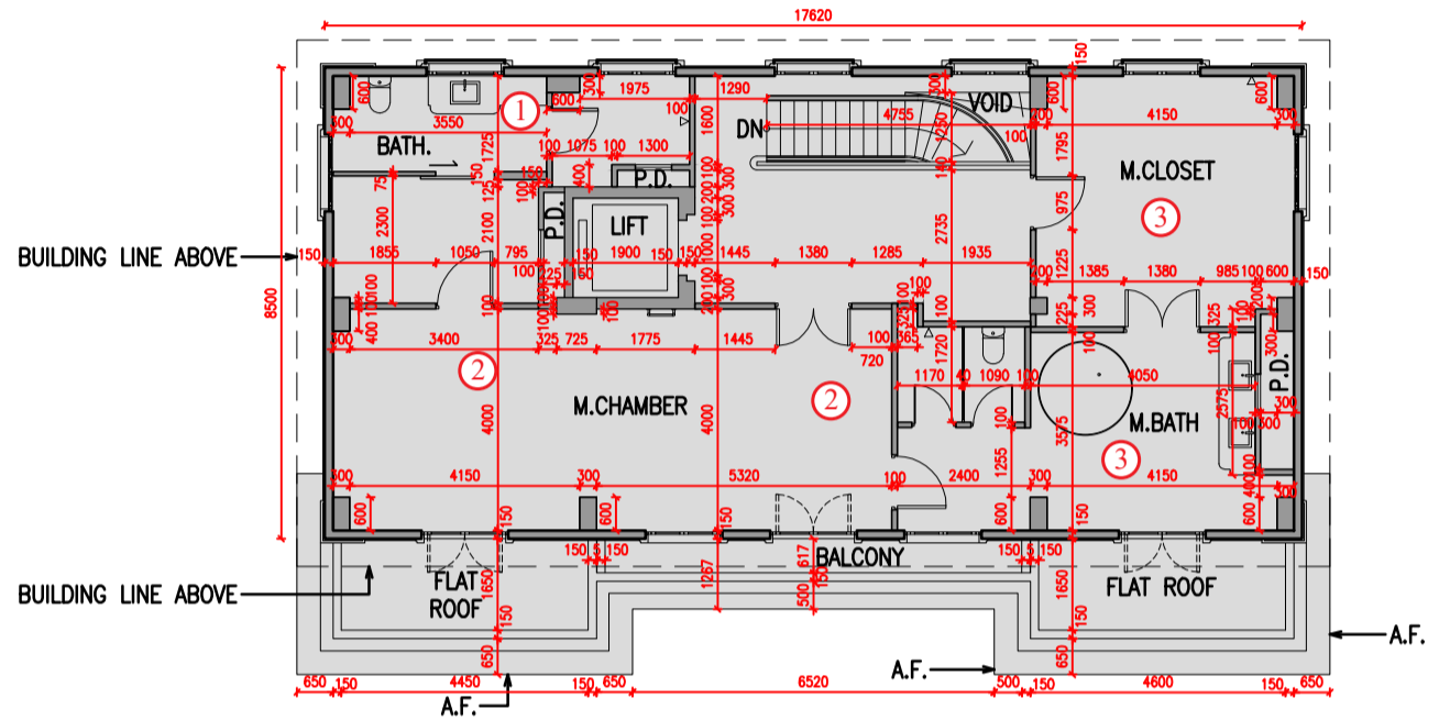
2/F FLOOR PLAN SHOWING AS-IS LAYOUT
