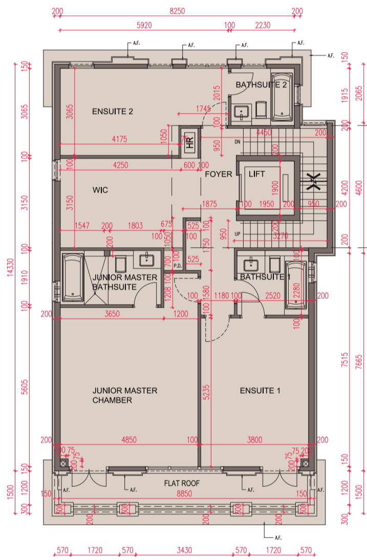
FIRST FLOOR PLAN 一樓平面圖
