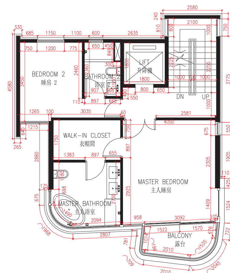
2/F For House E E座洋房2樓
