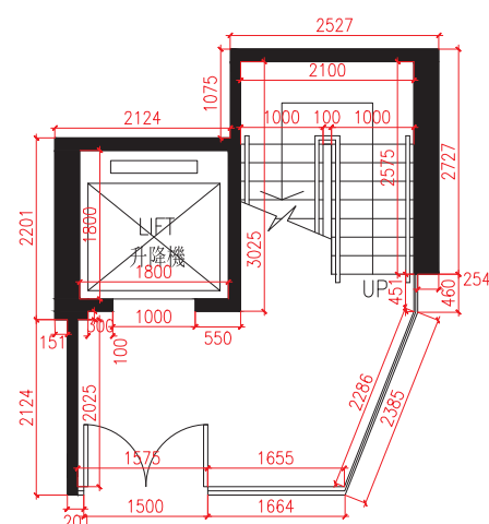
Lift Lobby on Carport Floor for House J J座車庫層之入口大堂
