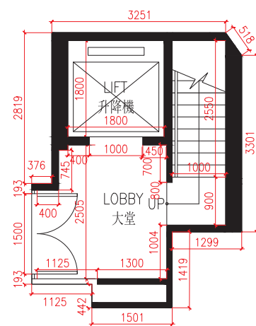
Lift Lobby on Carport Floor for House M M座車庫層之入口大堂
