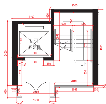
Lift Lobby on Carport Floor for House L L座車庫層之入口大堂
