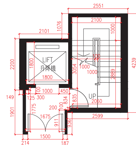
Lift Lobby on Carport Floor for House C C座車庫層之入口大堂
