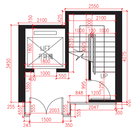
Lift Lobby on Carport Floor for House I I座車庫層之入口大堂
