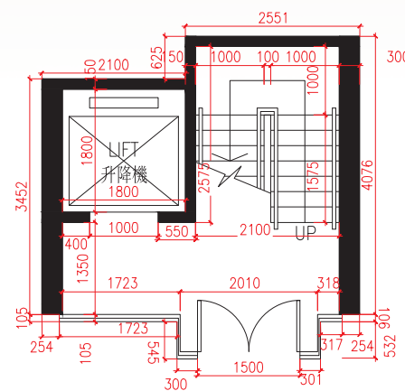
Lift Lobby on Carport Floor for House G G座車庫層之入口大堂
