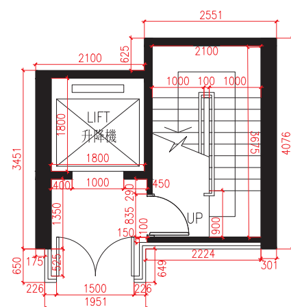
Lift Lobby on Carport Floor for House B B座車庫層之入口大堂
