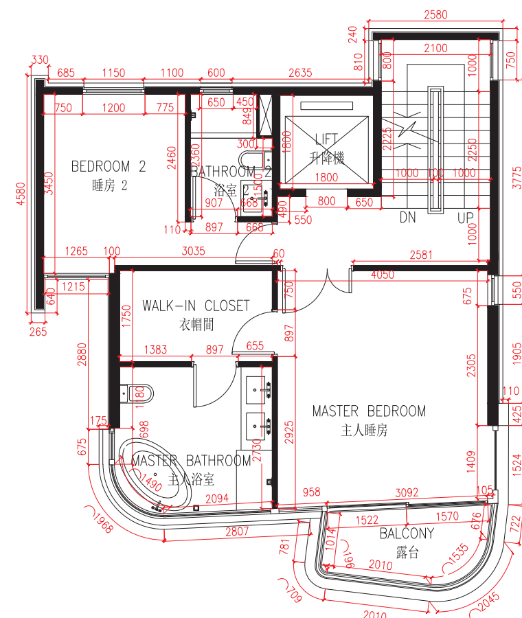
2/F For House D D座洋房2樓
