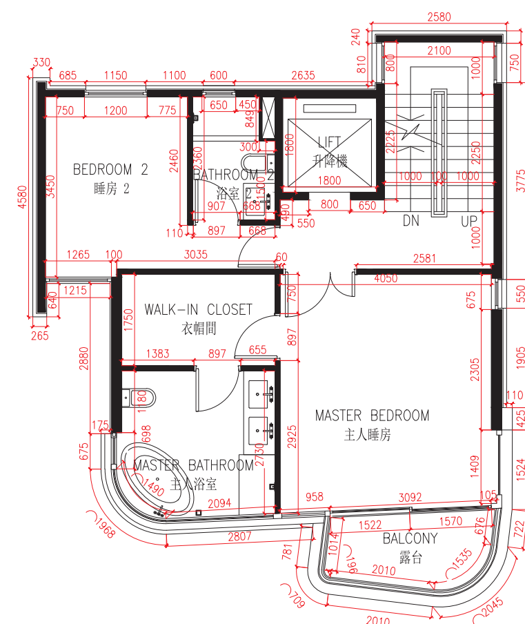
2/F For House C C座洋房2樓
