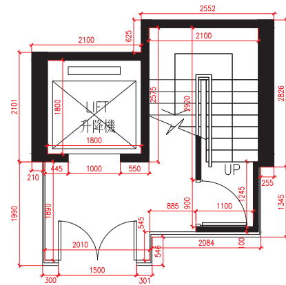
Lift Lobby on Carport Floor for House K K座車庫層之入口大堂
