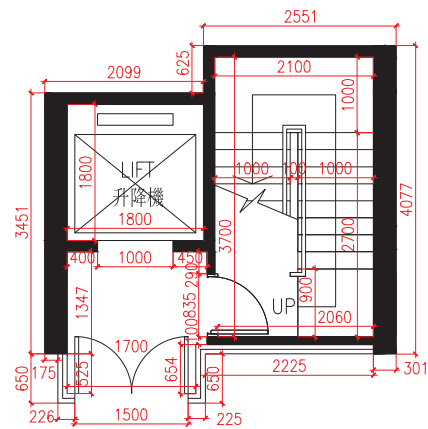
Lift Lobby on Carport Floor for House D D座車庫層之入口大堂
