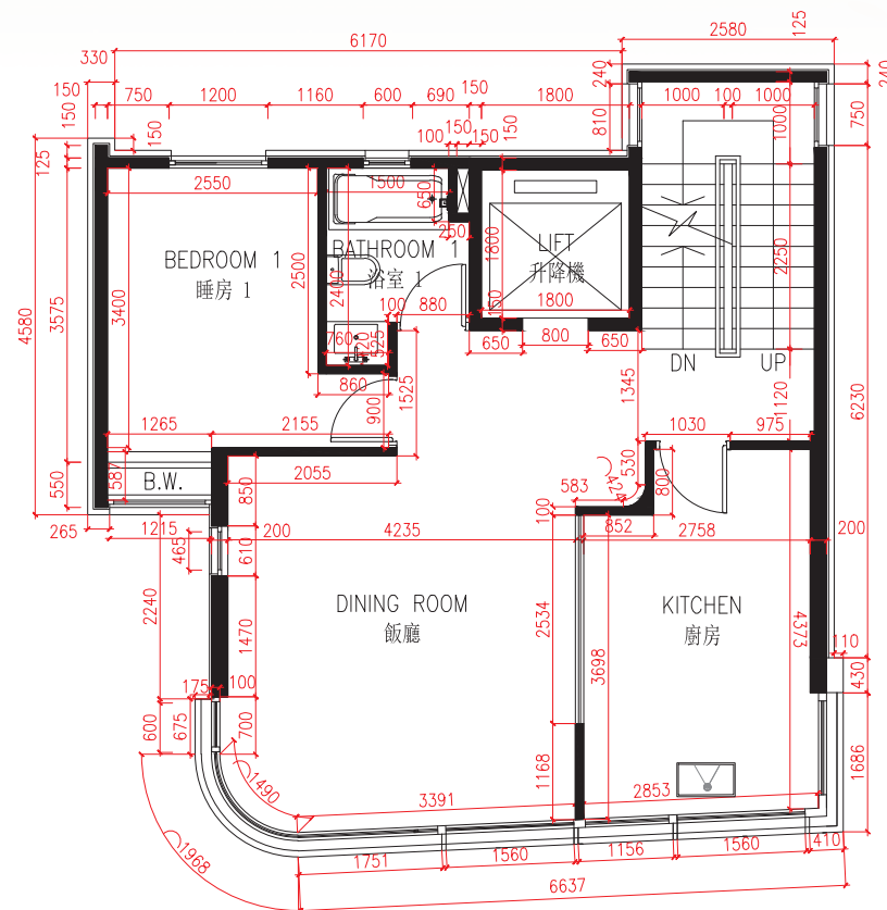
1/F For House H H座洋房1樓
