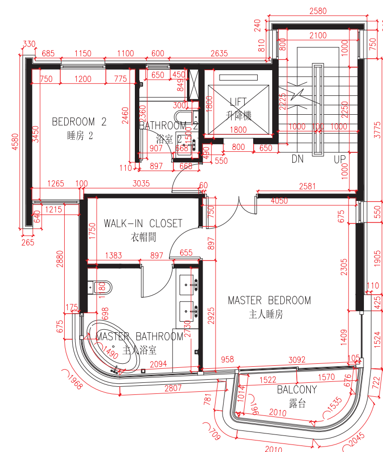
2/F For House B B座洋房2樓
