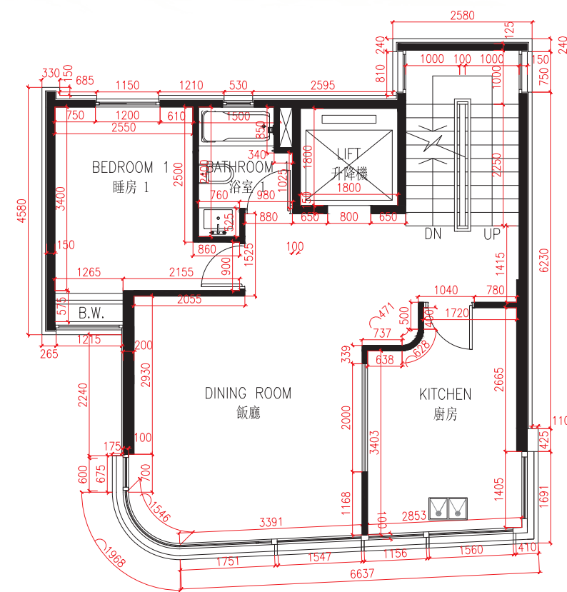
1/F For House I I座洋房1樓
