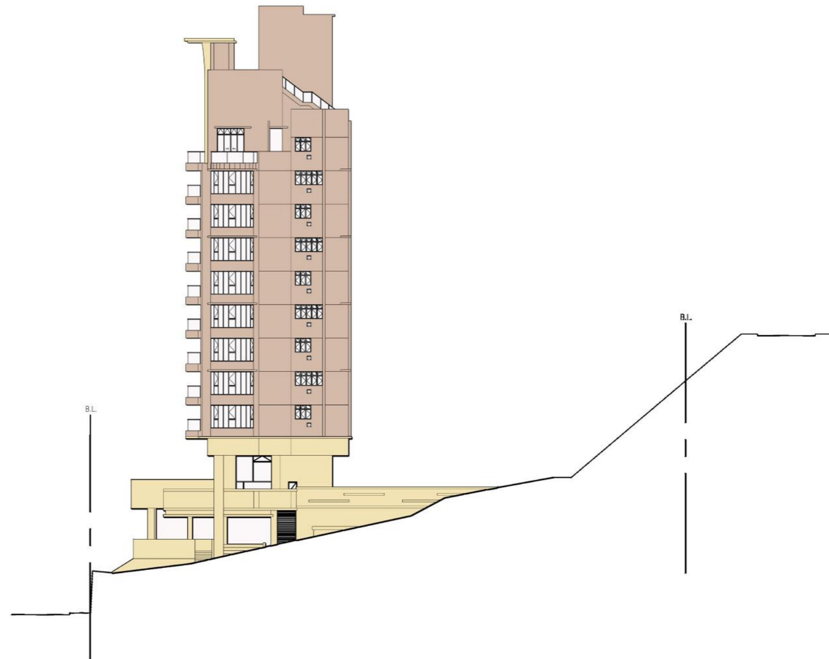
Elevation Plan of Tower (East) 大廈立面圖 (東面)
