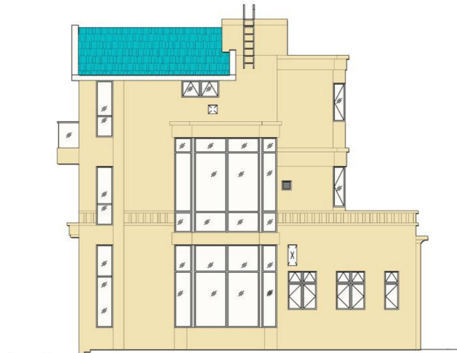
Elevation Plan (East) 立面圖 (東面)
