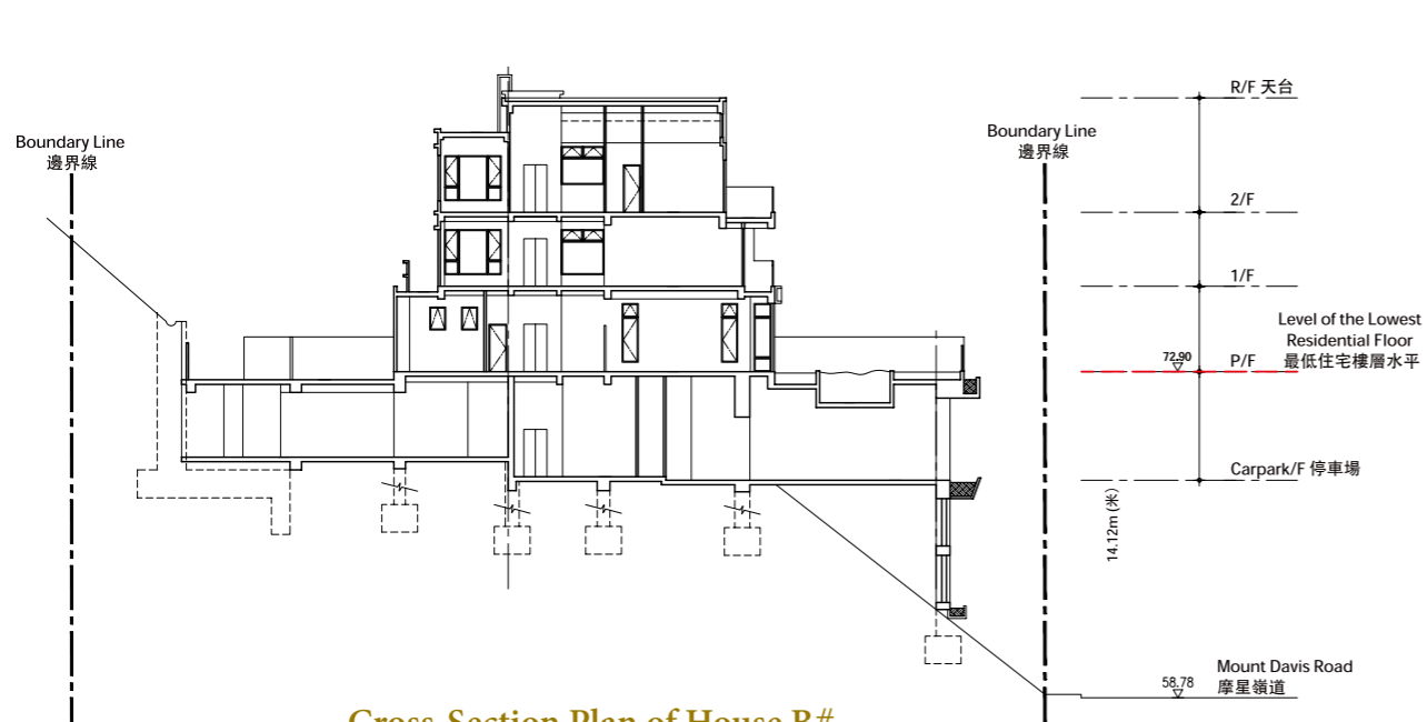
Cross-Section Plan of House B# 洋房 B 截面圖#
