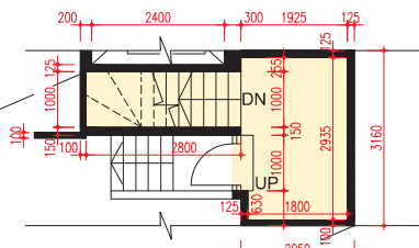
PART PLAN OF STAIRCASE FOR 16/F FLAT A
