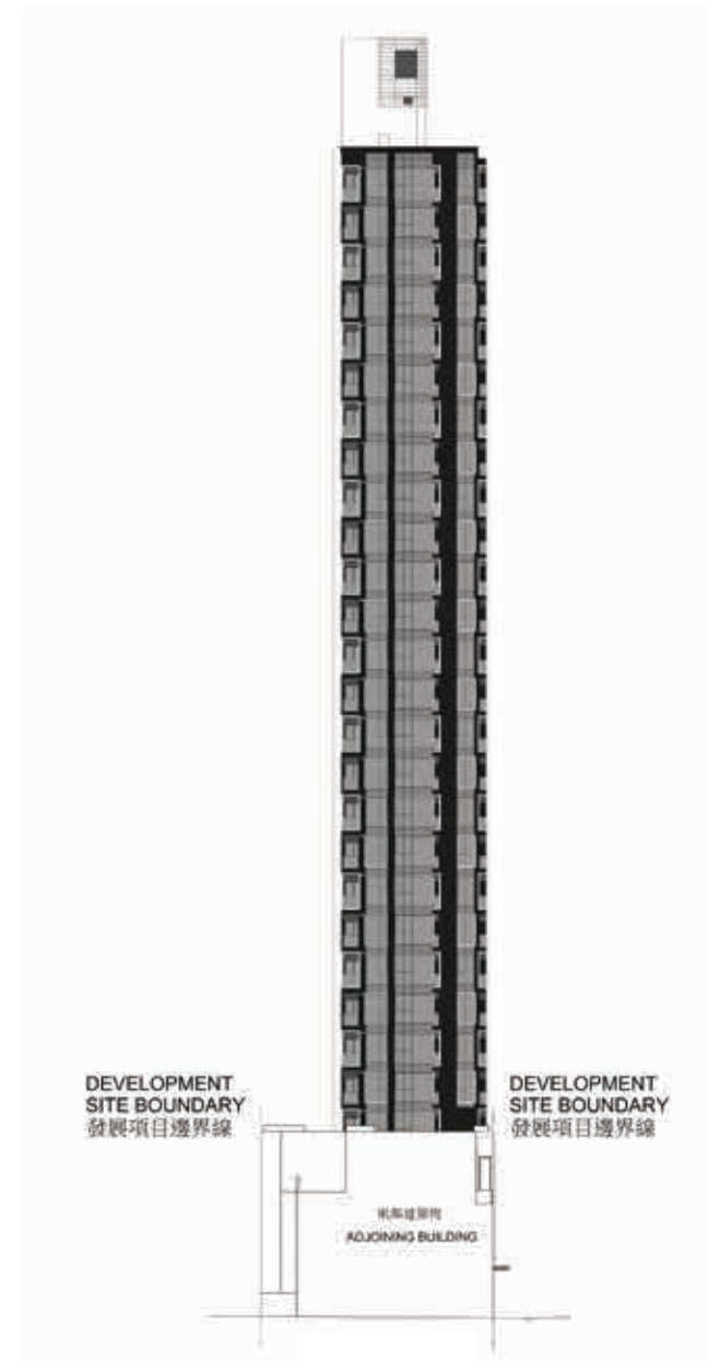
西北立面圖 North-West Elevation
