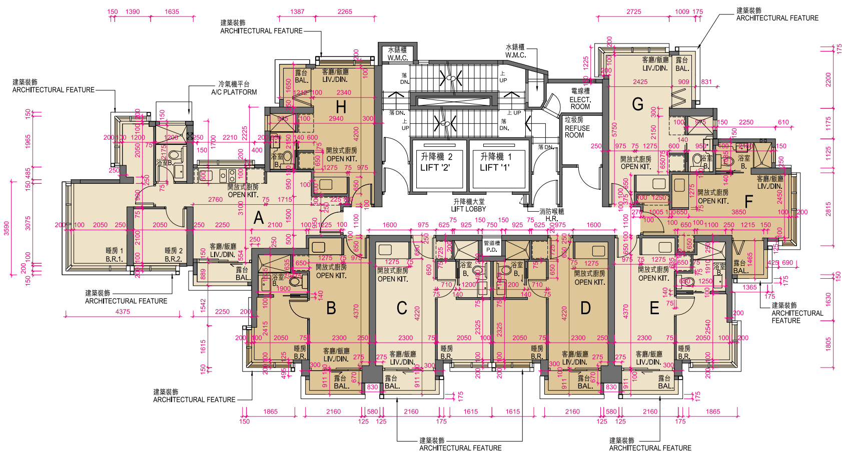
5樓、7樓及9樓平面圖 5th, 7th & 9th FLOOR PLAN
