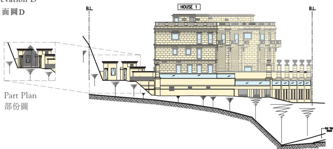
Elevation D
