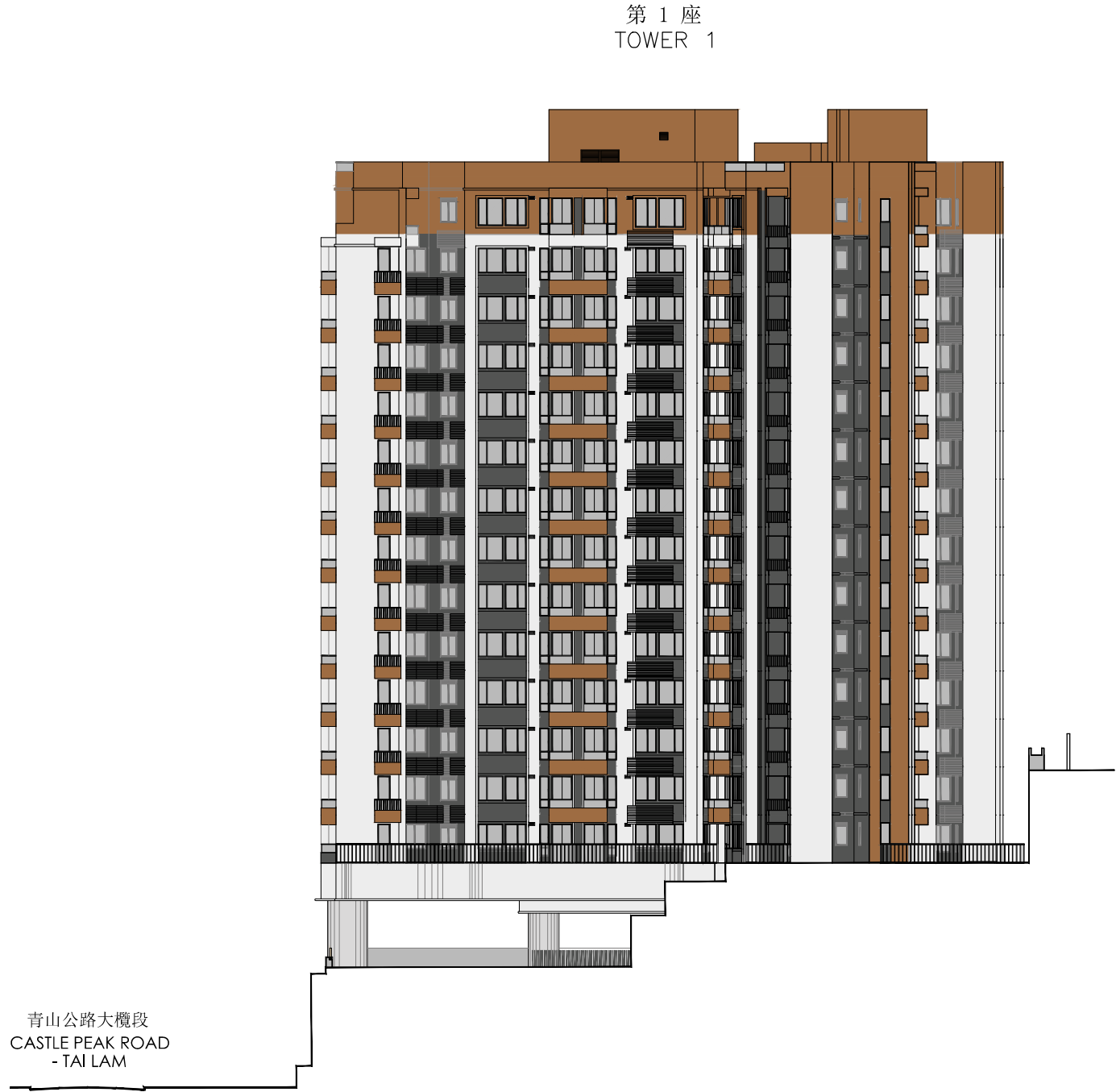
立面圖4 Elevation plan 4
