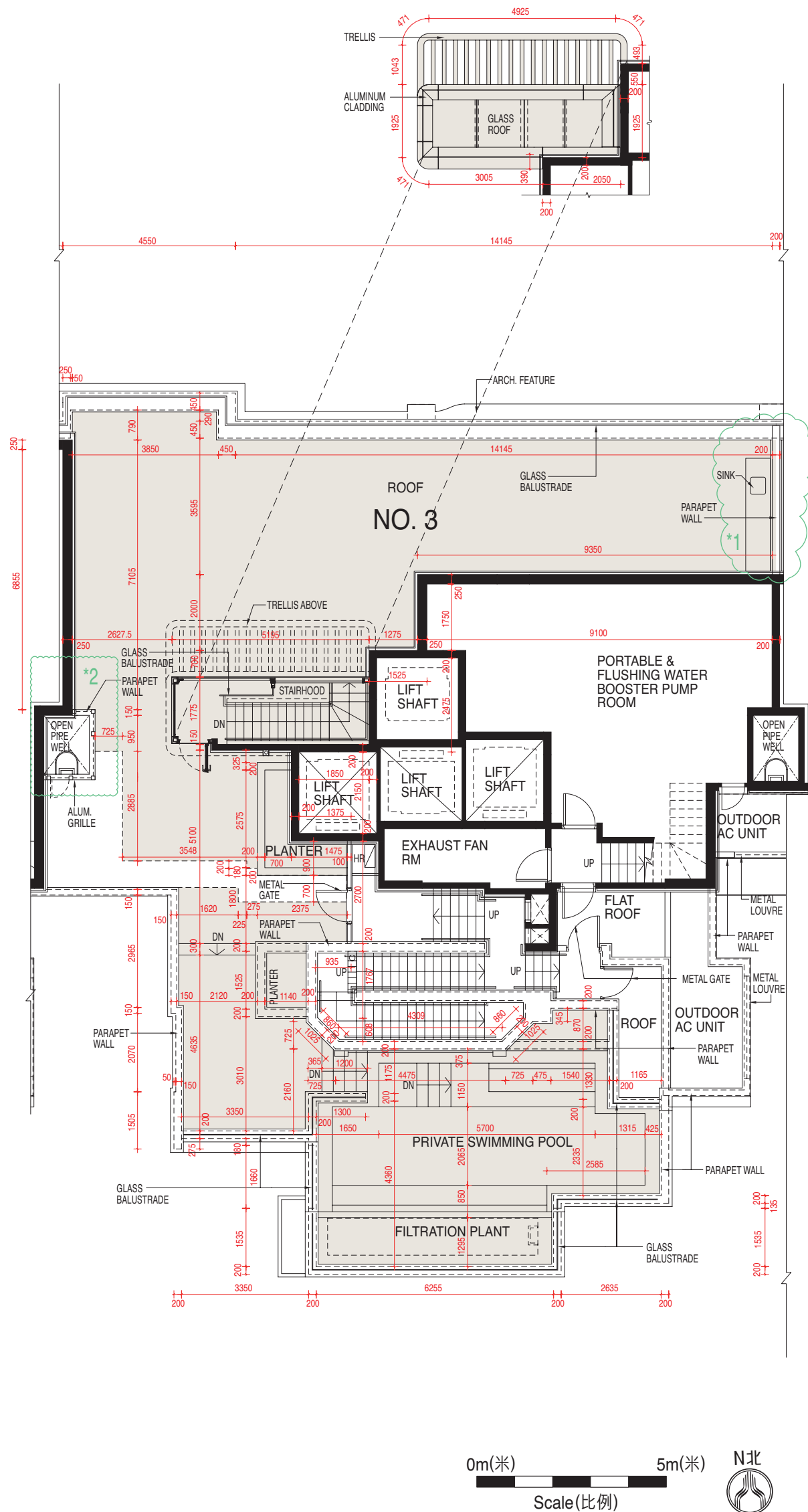
3號現狀間隔平面圖 Floor plan of No.3 showing latest layout
