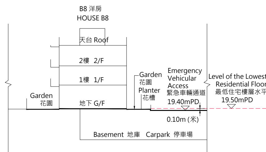
Cross-section Plan B8 橫截面圖 B8
