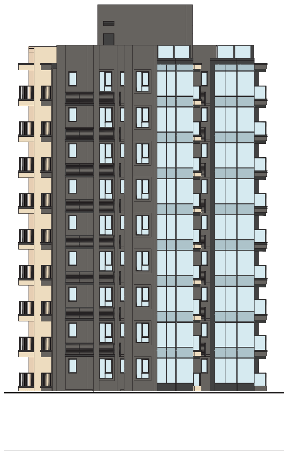
Elevation Plan C3 立面圖 C3
