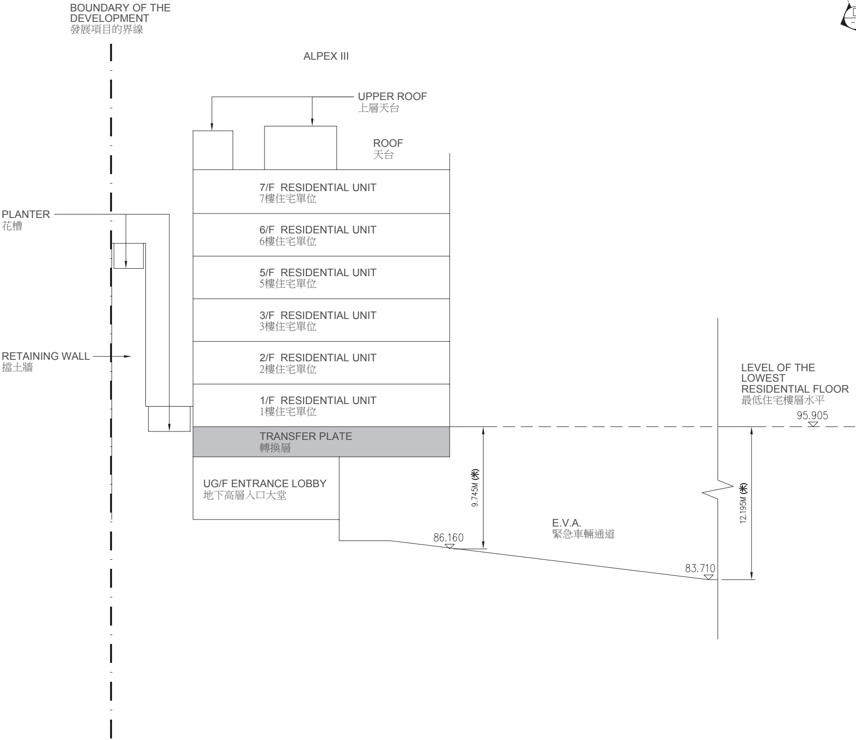
CROSS-SECTION D
