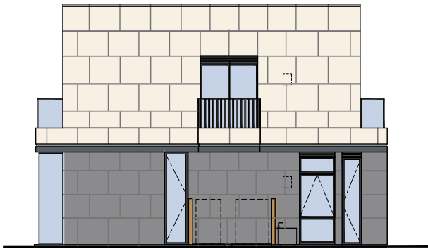
Elevation Plan 8 立面圖八
