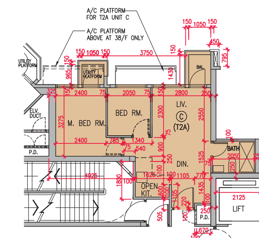
Part Plan of Tower 2 (2A) Unit C on 38/F
