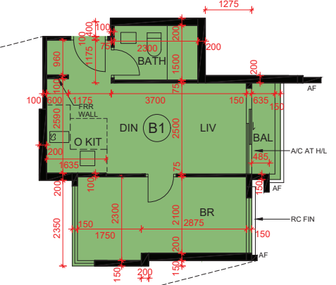
PART PLAN AT 2/F-3/F AND 5/F 2樓至3樓 及 5樓部份平面圖
