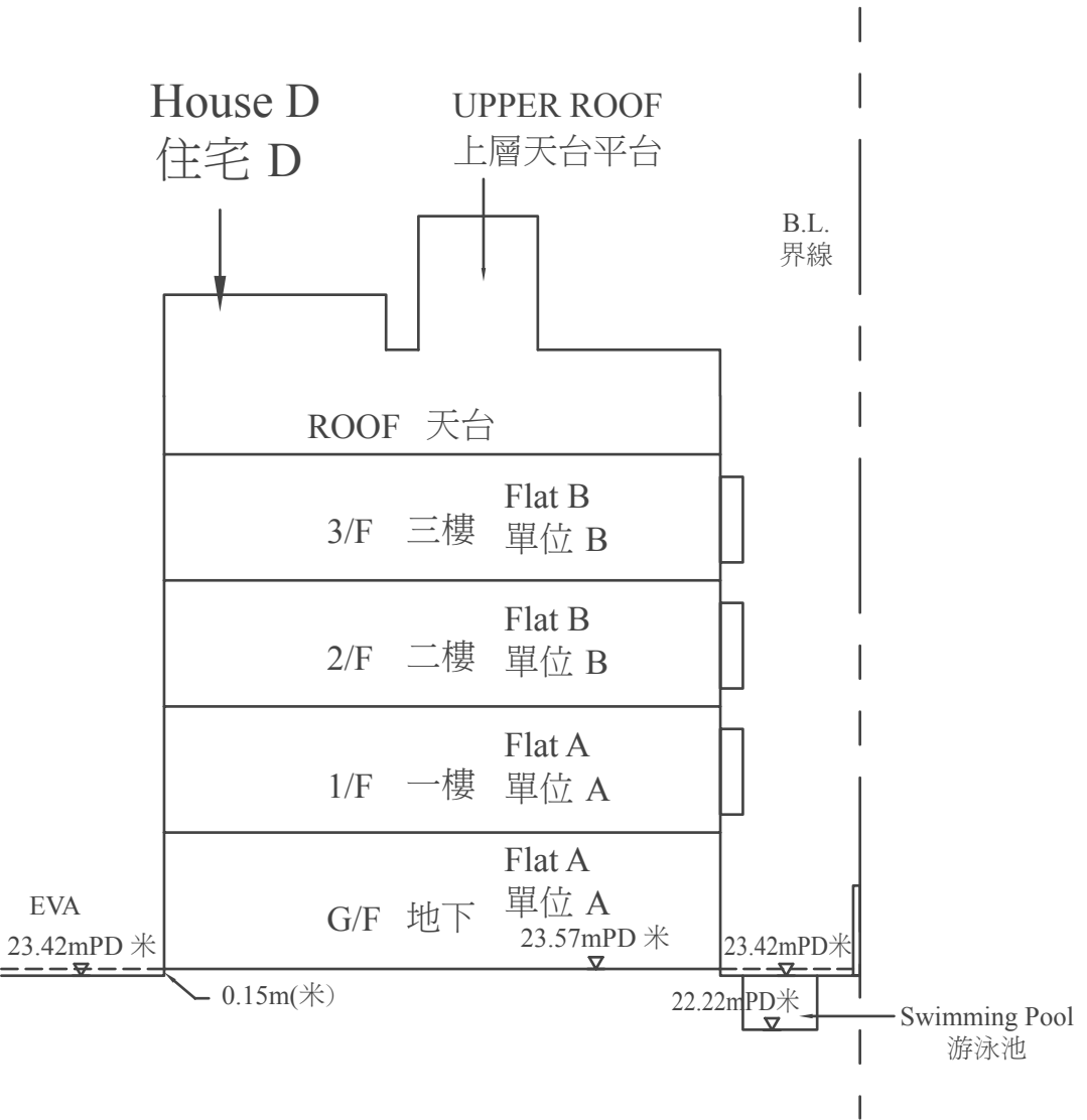
Cross-Section F-F 橫截面圖F-F
