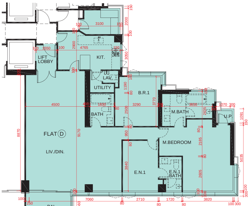
9/F FLAT D FLOOR PLAN 9樓單位D平面圖
