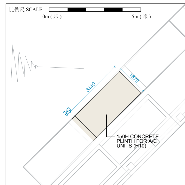
10號洋房地主層部分平面圖二 Part Plan 2 For House 10 Master Ground Floor Plan
