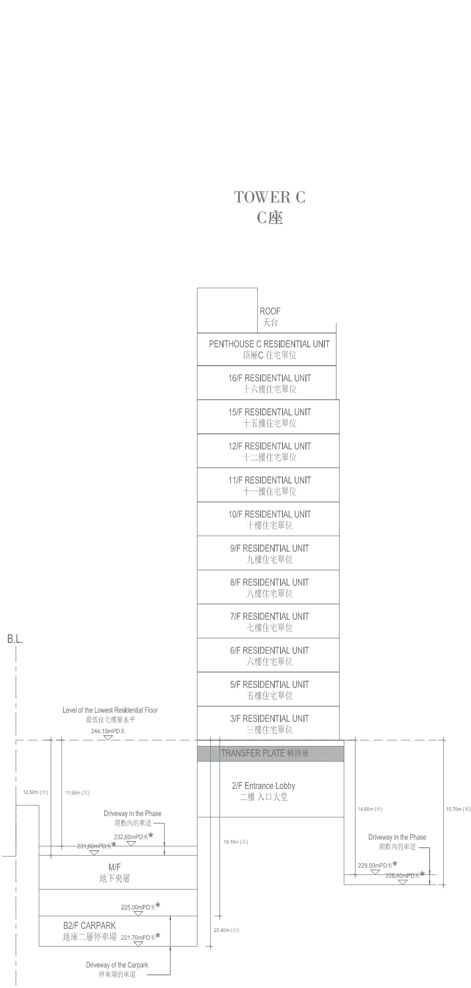
Section B 剖面圖B
