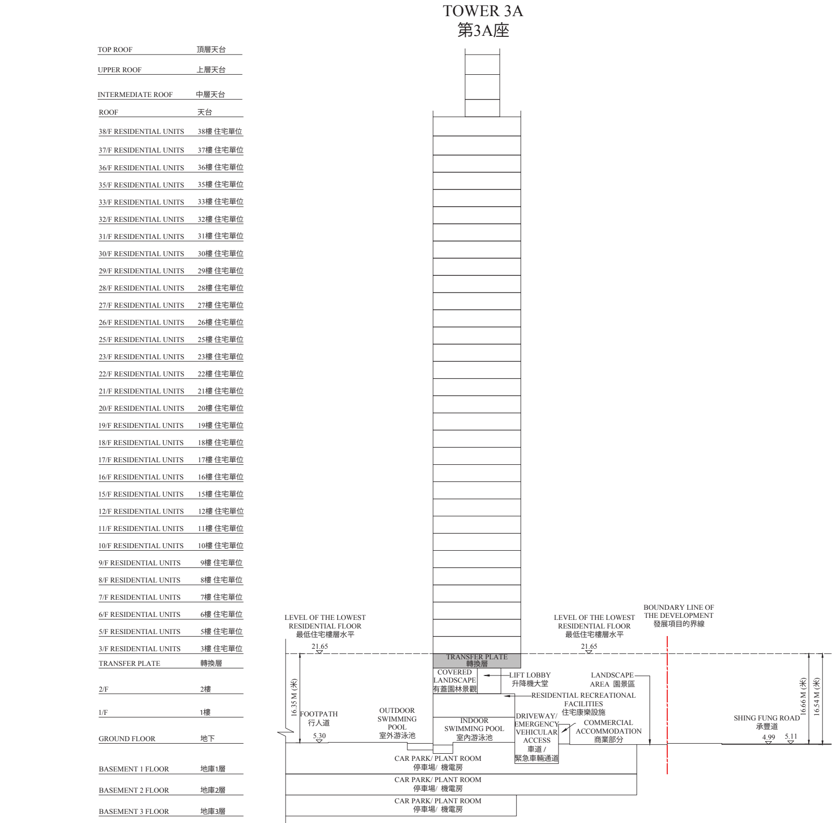
CROSS-SECTION PLAN E - E 橫截面圖 E - E
