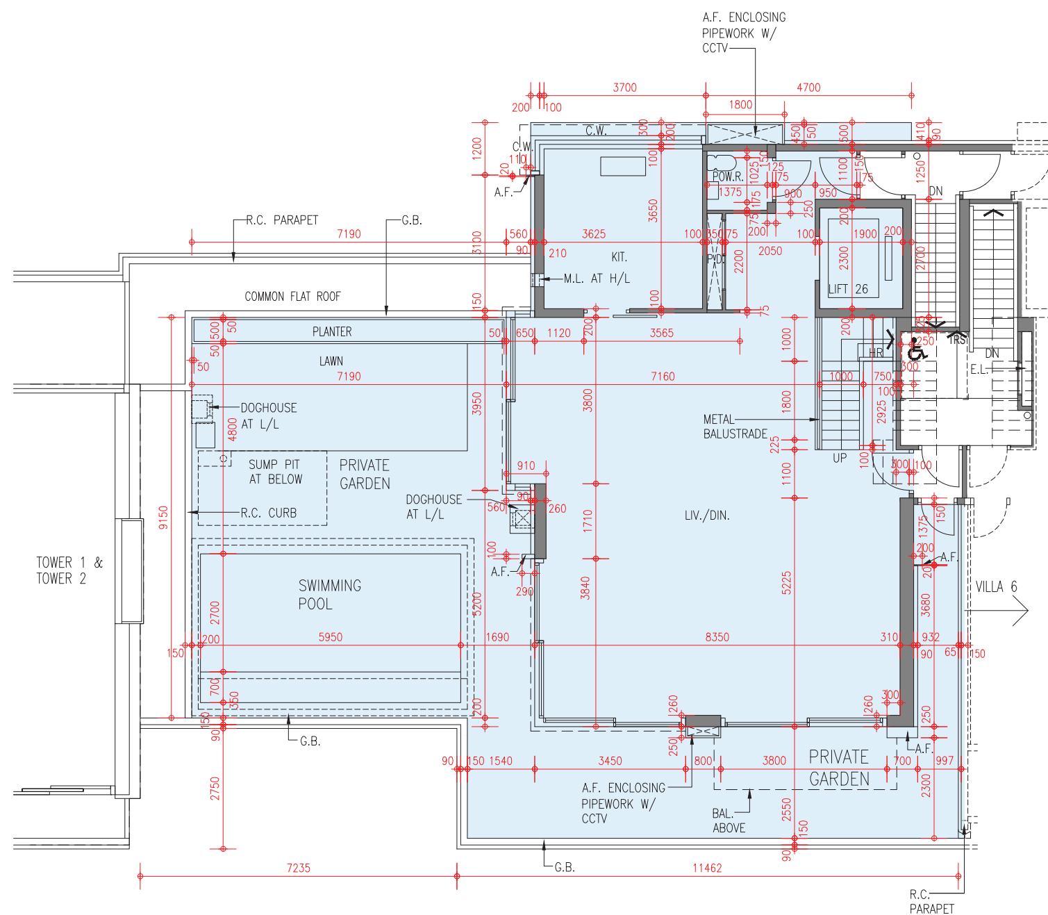
3/F Floor Plan 3樓樓面平面圖
