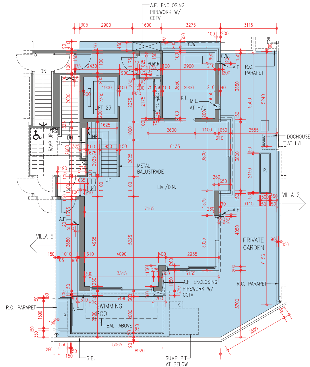
3/F Floor Plan 3樓樓面平面圖
