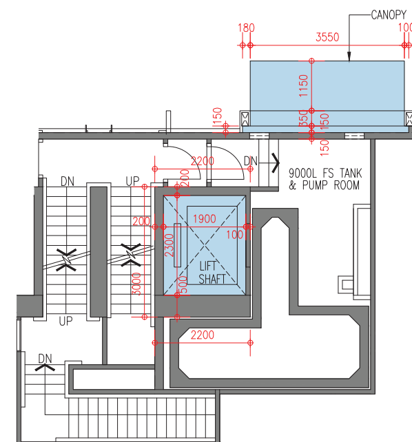
1/F Floor Plan
