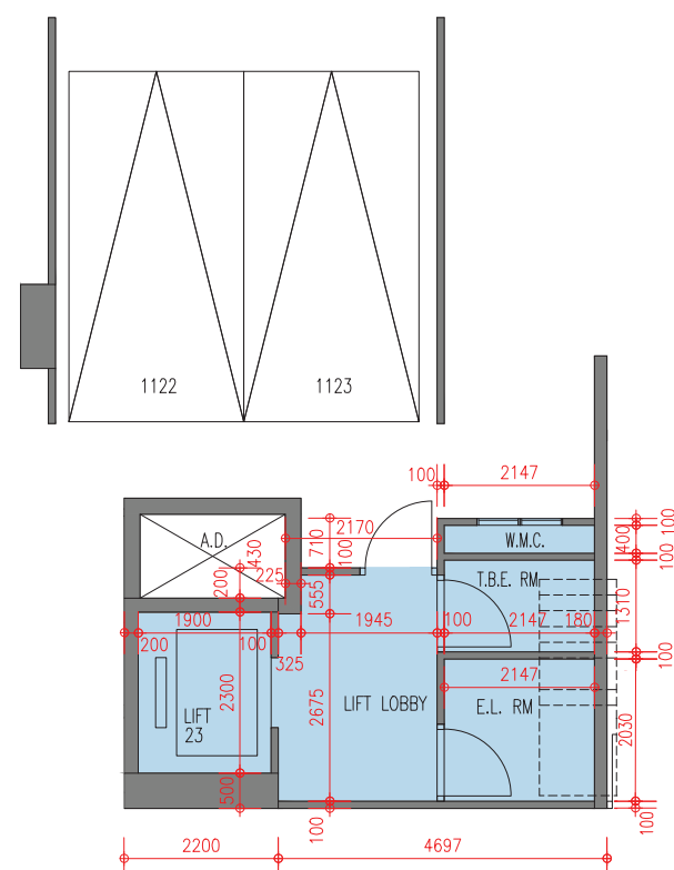
Basement 1 Floor Plan
