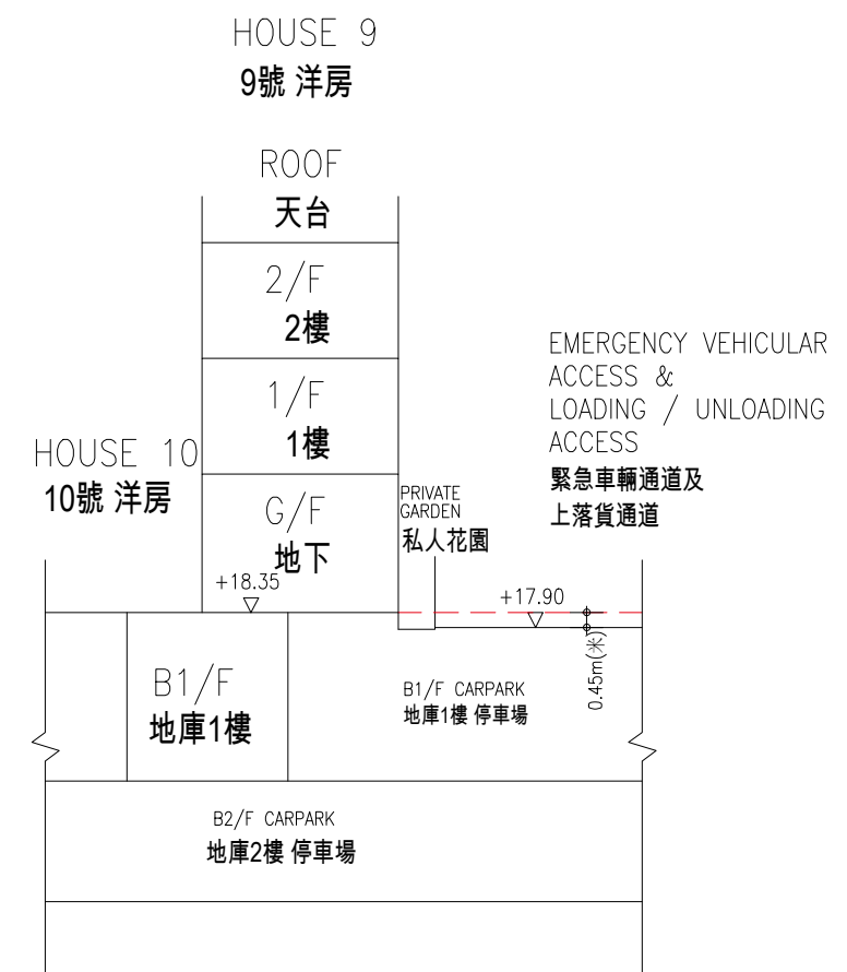
Cross-Section Plan H9b 橫截面圖 H9b
