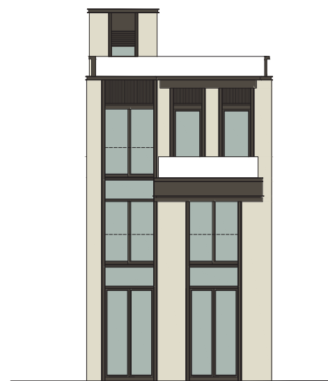
立面圖 B (適用於 A1, A2, A5, A10, B3, B6, C1, C5 及 C6 洋房) Elevation B (For Houses A1, A2, A5, A10, B3, B6, C1, C5 and C6)
