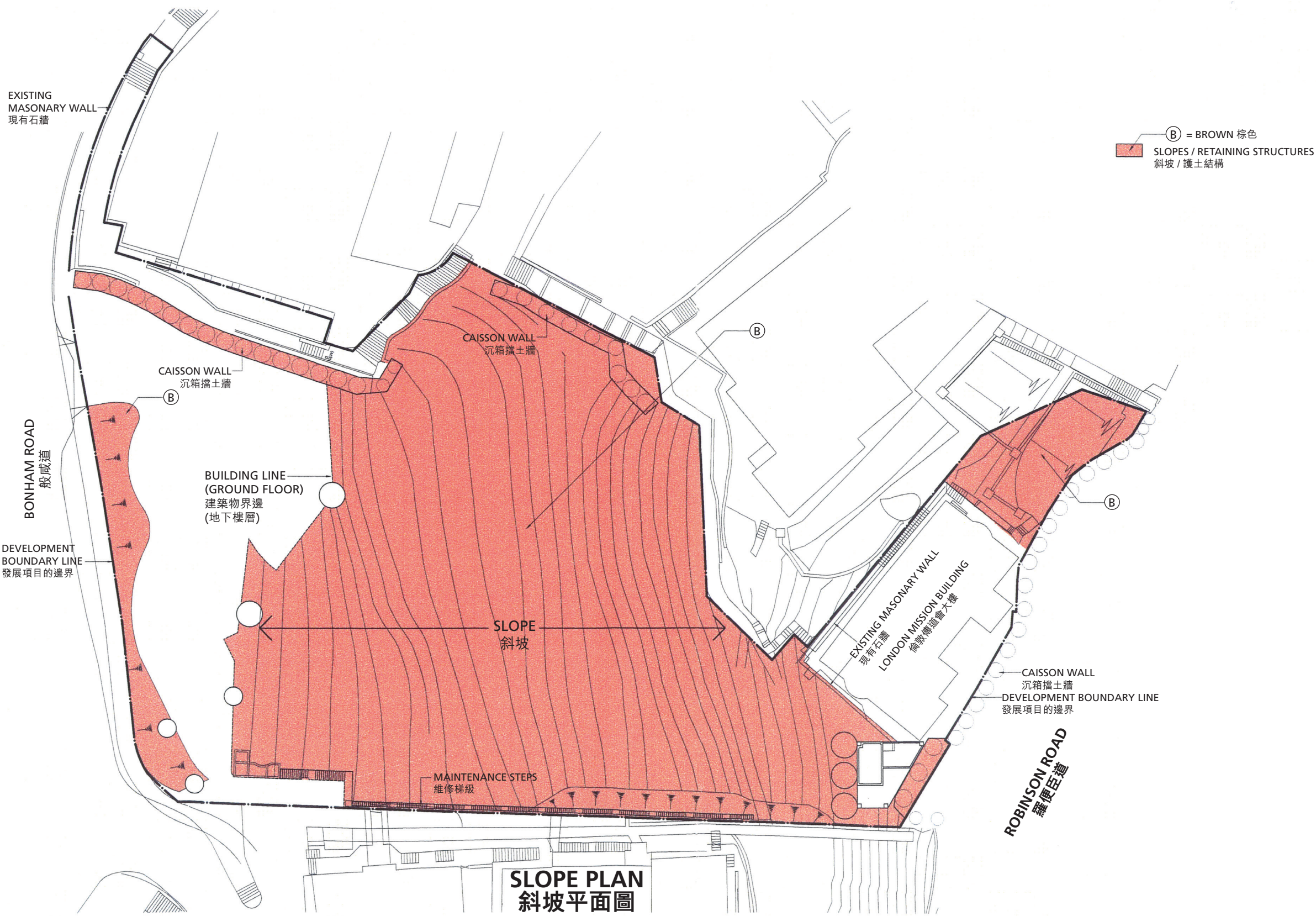
Slope and Retaining Structures Plan 斜坡及護土結構圖
