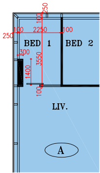
Part Plan of Flat A of 81/F-83/F and 85/F. of Zone 1 of Tower 20* 第20座，第1區，81樓至83樓及85樓A室部分平面圖*
