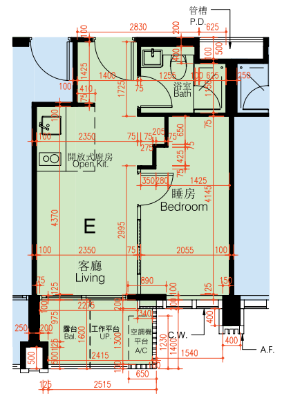
18/F Flat E Floor Plan 18樓單位E平面圖
